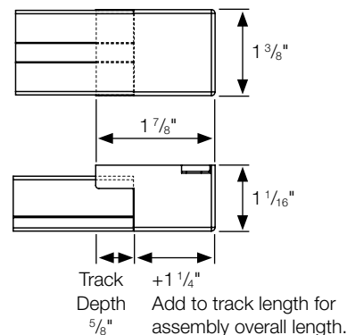
Return Pulley RTMDSS50RP
