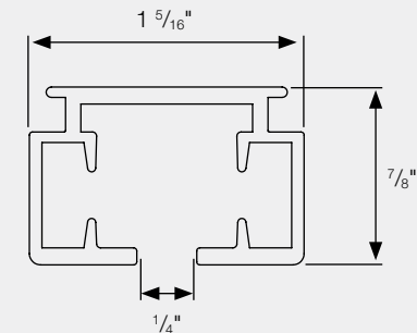
SHC Heavy Duty Track
