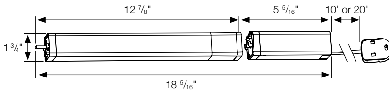
Slim Line Drapery Motor with 110v AC / DC Power Transformer RTMLDSS50 with RTMDSSPT 10' (plug RTMP included) or RTMLDSS50 with RTMDSSPTCS 20' (plug RTMP not included)
