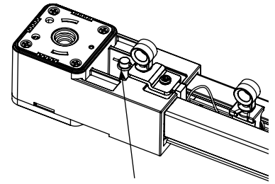
RIPPLEFOLD: Place the cord & attachment tab under the End Stop and tighten the fastener.
